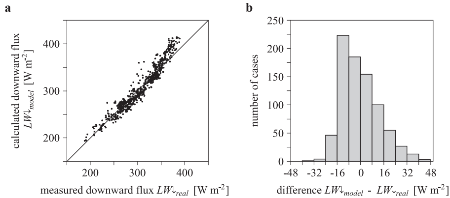
Figure 6. Comparison of measured values of the downward longwave radiation flux LW\downarrow_{real} with values LW\downarrow_{model} calculated using eq. (5) for all sky conditions (a); error histogram (b)
