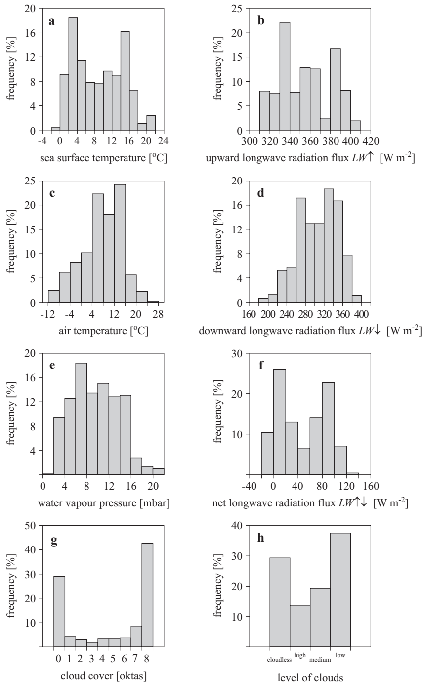
Figure 1. Characteristics of the empirical data gathered in the southern Baltic and Baltic Proper: sea surface temperature (a); upward longwave radiation (b); air temperature (c); downward longwave radiation (d); water vapour pressure (e); net longwave radiation (f); cloud cover (g); cloud level (h)
