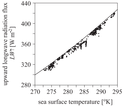
Figure 2. Empirical relationship of the upward radiation flux LW \uparrow and surface water temperature in the Baltic Sea. The solid line was calculated from the Stefan-Boltzmann law
