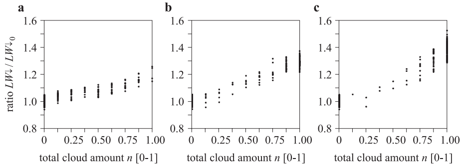
Figure 7. Empirical dependence on the total cloud amount n of the ratio of the downward longwave radiation flux for all sky conditions LW \downarrow to the downward flux from a cloudless atmosphere LW \downarrow_0 calculated from eq. (4): low-level clouds (a), mid-level clouds (b), high-level clouds (c)
