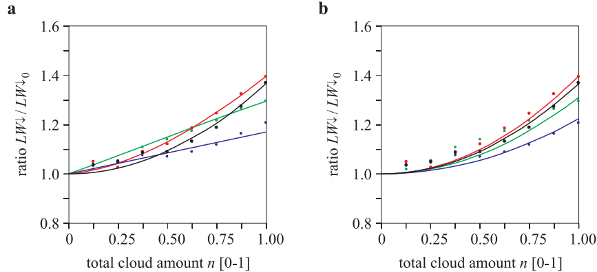
Figure 8. Mean values for particular cloud cover states of the ratio of the downward longwave radiation flux for all sky conditions LW \downarrow to the downward longwave radiation flux from a cloudless atmosphere LW \downarrow_0 calculated from eq. (4) in relation to the total cloud amount n . The plots represent functions with different coefficients \gamma_i (see eq. (6) and Table 3), which best approximate the above relationship for: low-level clouds – red line, mid-level clouds – green line, high-level clouds – blue line (a); the same for the quadratic function (b). The solid black line is calculated from eq. (5)
