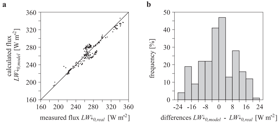
Figure 4. Comparison of measured values of the downward longwave radiation flux from a cloudless atmosphere LW_{\downarrow,real} with values of LW_{\downarrow,model} calculated according to eq. (4) (a), and the histogram of the differences between these two values (b)
