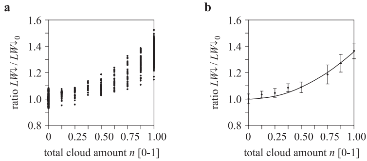
Figure 5. Empirical dependence on the total cloud amount n of the ratio of the downward longwave radiation flux for all sky conditions LW\downarrow to the downward flux from a cloudless atmosphere LW\downarrow_0 calculated from eq. (4) (a); the same for averaged values and standard deviations of the total cloud amount in the various intervals of n (b). The solid line was calculated from eq. (5)
