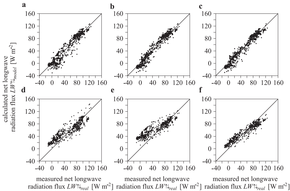
Figure 10. Comparison of values of the net longwave radiation flux LW \uparrow \downarrow_{real} measured in the Baltic with values of the flux LW \uparrow \downarrow_{model} calculated using the various formulas: formula (8) – eq. (Z1) (a); formula (8) – eq. (Z2) (b); formula (8) – eq. (Z3) (c); Clark et al. (1974) (d); Bignami et al. (1995) (e); Josey et al. 2003 – J03a (f)
