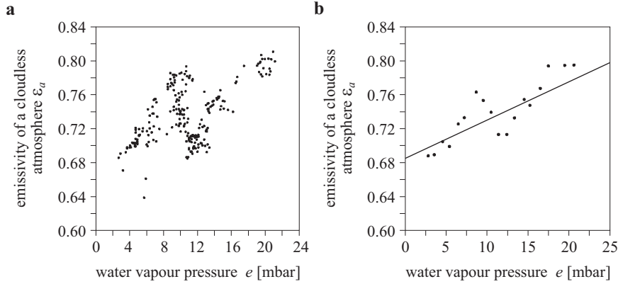
Figure 3. Empirical dependence of the emissivity of a cloudless atmosphere \varepsilon_a (see eqs. (3) and (4)) on the water vapour pressure e (a) and on the averaged values in the different intervals of the water vapour pressure e (b)
