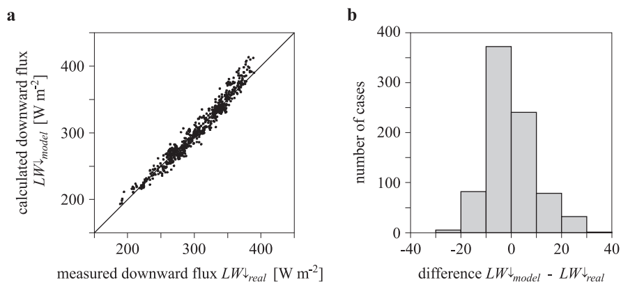
Figure 9. Comparison of measured values of the downward longwave radiation flux LW \downarrow_{real} with values LW \downarrow_{model} calculated using formula (6) with different \gamma_i (see column 2 in Table 3) (a), and error histogram (b), for all sky conditions
